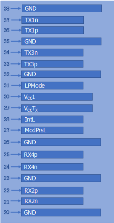
Top Board
