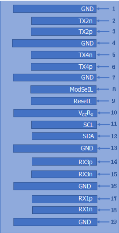
Bottom Board
